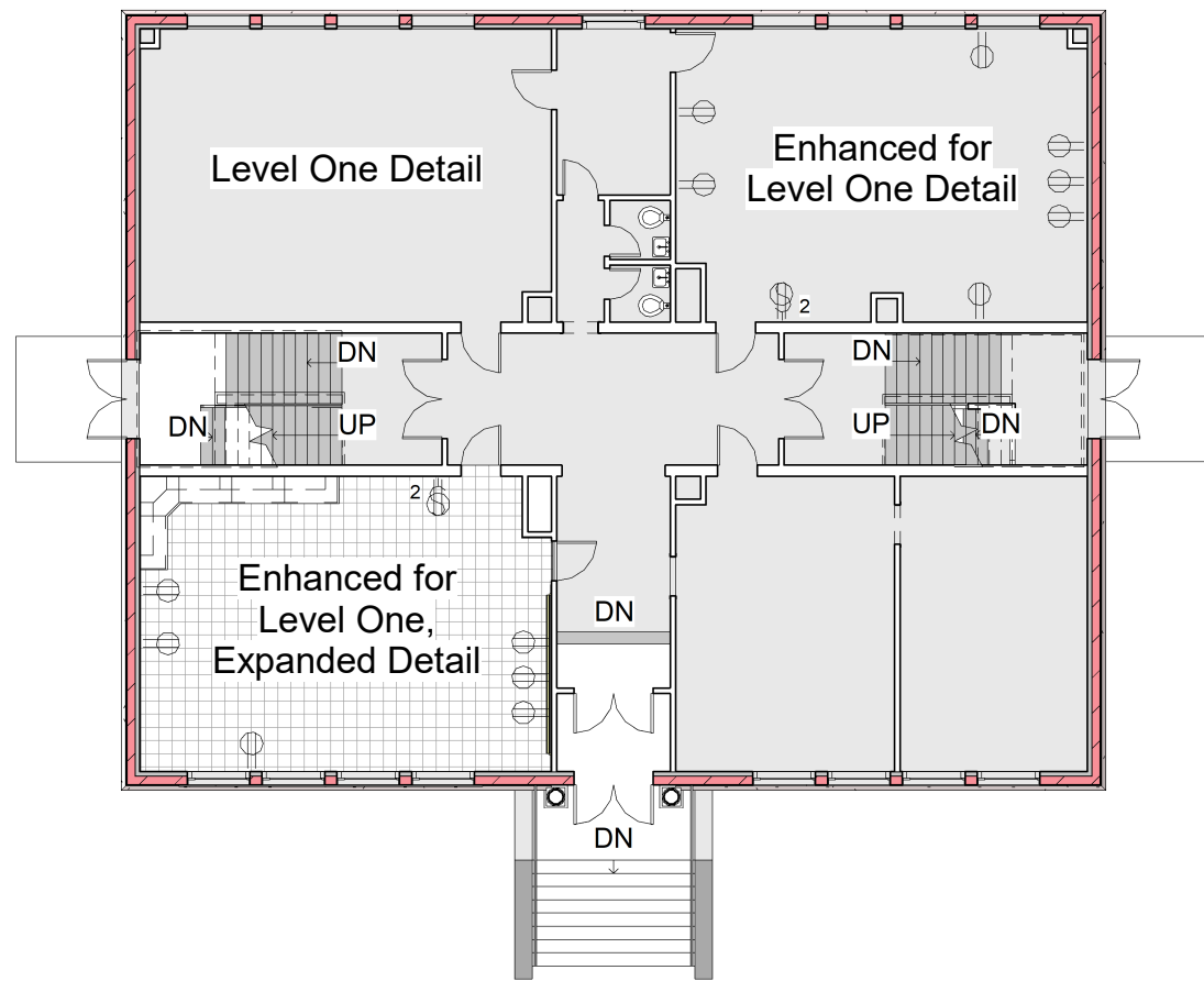
① First Floor Plan 1/16" = 1'-0"
