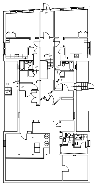
○ BASEMENT PLAN APARTMENT BUILDING 0 4 8 12 16
