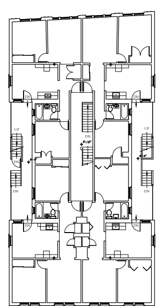
○ FIRST FLOOR PLAN APARTMENT BUILDING 0 4 8 12 16
